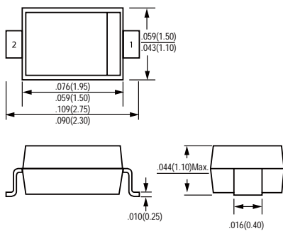
SOD-323
