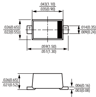
SOD-723
