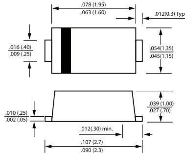
SOD-323L
