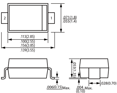
SOD-123
